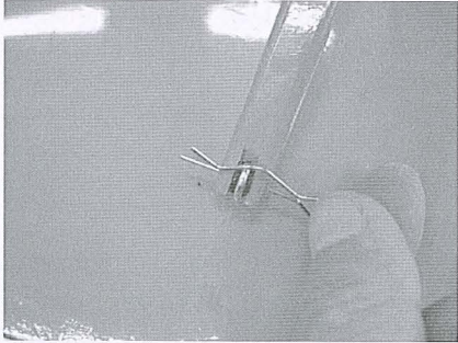
Connect the end of wing strut with eye screw on the main wing and secure with R pin.
