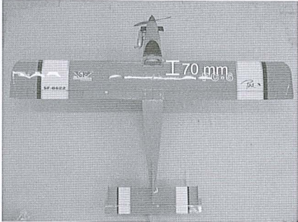
The recommended Center of Gravity location is 70mm back from the leading edge.
